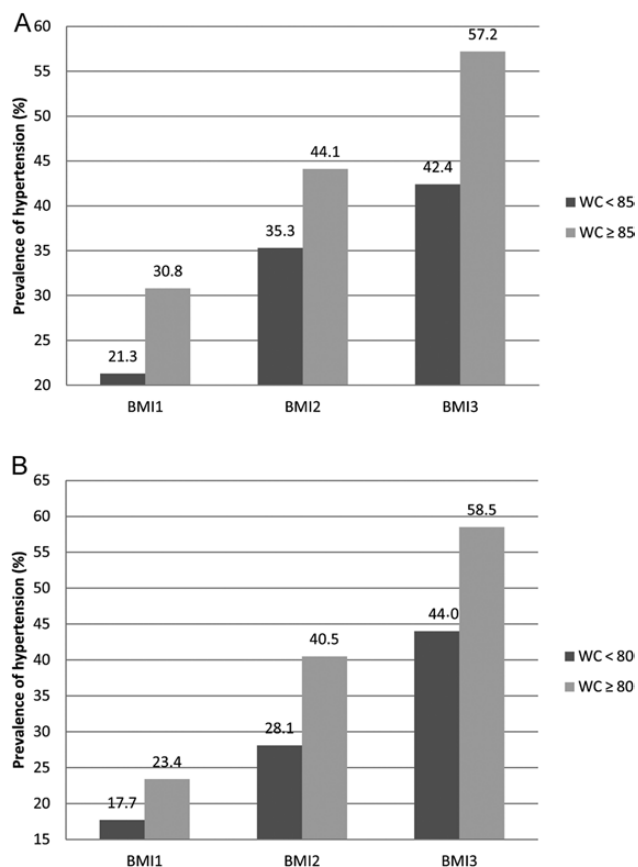
Figure 1. Prevalence of hypertension according to body mass index (BMI) and waist circumference (WC). (a) Men. (b) Women. BMI1, BMI2, and BMI3 correspond to BMIs of <23.9 kg/m 2 , 24.0–27.9 kg/m 2 , and ≥28.0 kg/m 2 , respectively.
