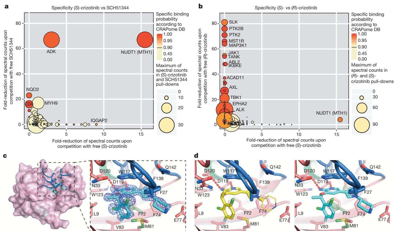
Figure 3 | Specificity and MTH1 co-crystal structure of (S)-crizotinib. a , Comparison of (S)-crizotinib specificity versus SCH51344 ( a ) and (R)-crizotinib ( b ). MTH1 is the only shared target with SCH51344 and is specific to (S)-crizotinib when compared to (R)-crizotinib. Data represent two independent experiments for each condition ( n = 2 per condition), and each replicate was analysed in two technical replicates. c , Co-crystal structure of (S)-crizotinib and MTH1. MTH1 is in pink with light green \alpha -helices and
