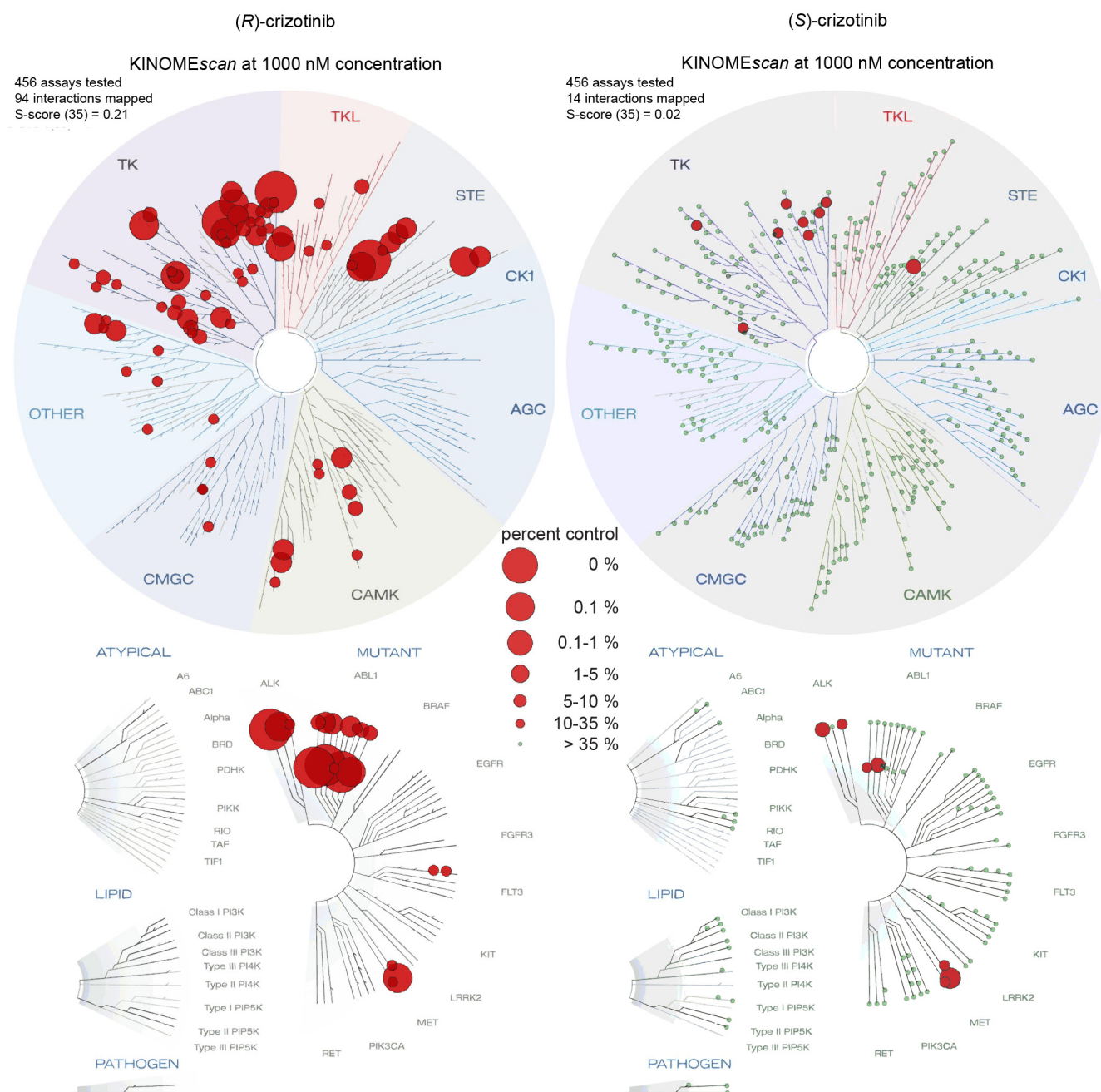
Extended Data Figure 3 | KINOMEScan results for both crizotinib enantiomers. Screening of both (R)- and (S)-crizotinib against a panel of 456 recombinant human protein kinases indicates a marked difference in the ability of the two enantiomers to bind kinases. (R)-crizotinib has high affinity towards a large number of kinases, including its cognate targets MET, ALK and
