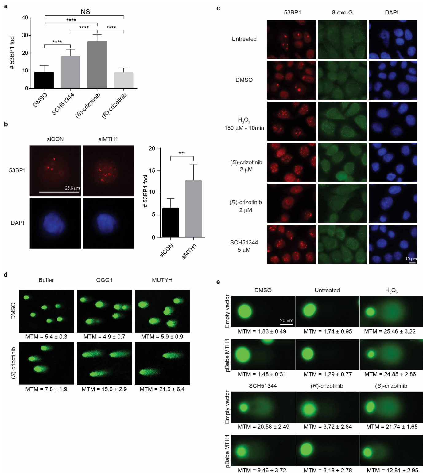
Extended Data Figure 6 | MTH1 suppression by siRNA or small-molecule inhibitors induces DNA damage. a , Quantification of 53BP1 foci formation in SW480 cells upon MTH1 inhibitor treatment. Concentrations are 5 \mu M for SCH51344 and 2 \mu M for each crizotinib enantiomer. Data are shown as mean \pm s.d. ( n = 3 ). Asterisks indicate significance by two-way ANOVA; NS, not significant. b , In line with results obtained for the MTH1 inhibitors SCH51344 and (S)-crizotinib, transient knockdown of MTH1 also induces formation of 53BP1 foci in SW480 cells. Images are representative and data are shown as mean \pm s.d. based on three independent experiments ( n = 3 ) ( P < 0.05 , t -test). c , Formation of 53BP1 foci correlates with increased 8-oxo-guanine staining in SW480 cells treated with the MTH1 inhibitors SCH51344
