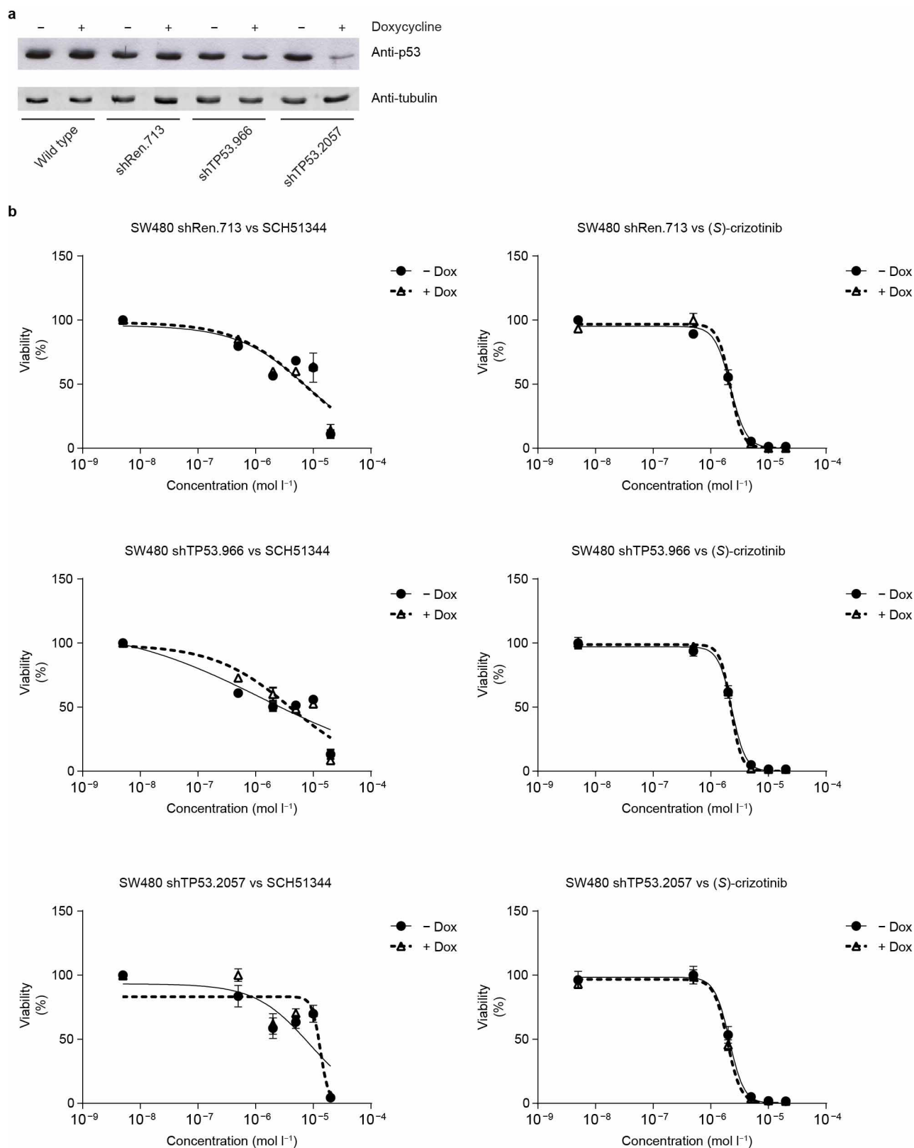
Extended Data Figure 7 | MTH1 inhibitor efficacy is not affected by loss of p53. a , Western blot evaluation of p53-shRNA knockdown efficiency. b , Viability curves from colony formation assays of SW480 cells expressing inducible non-targeting (shRen.713), or targeting anti-p53 shRNAs. Cells were cultured for 2 days either with or without doxycycline, plated in triplicate in
