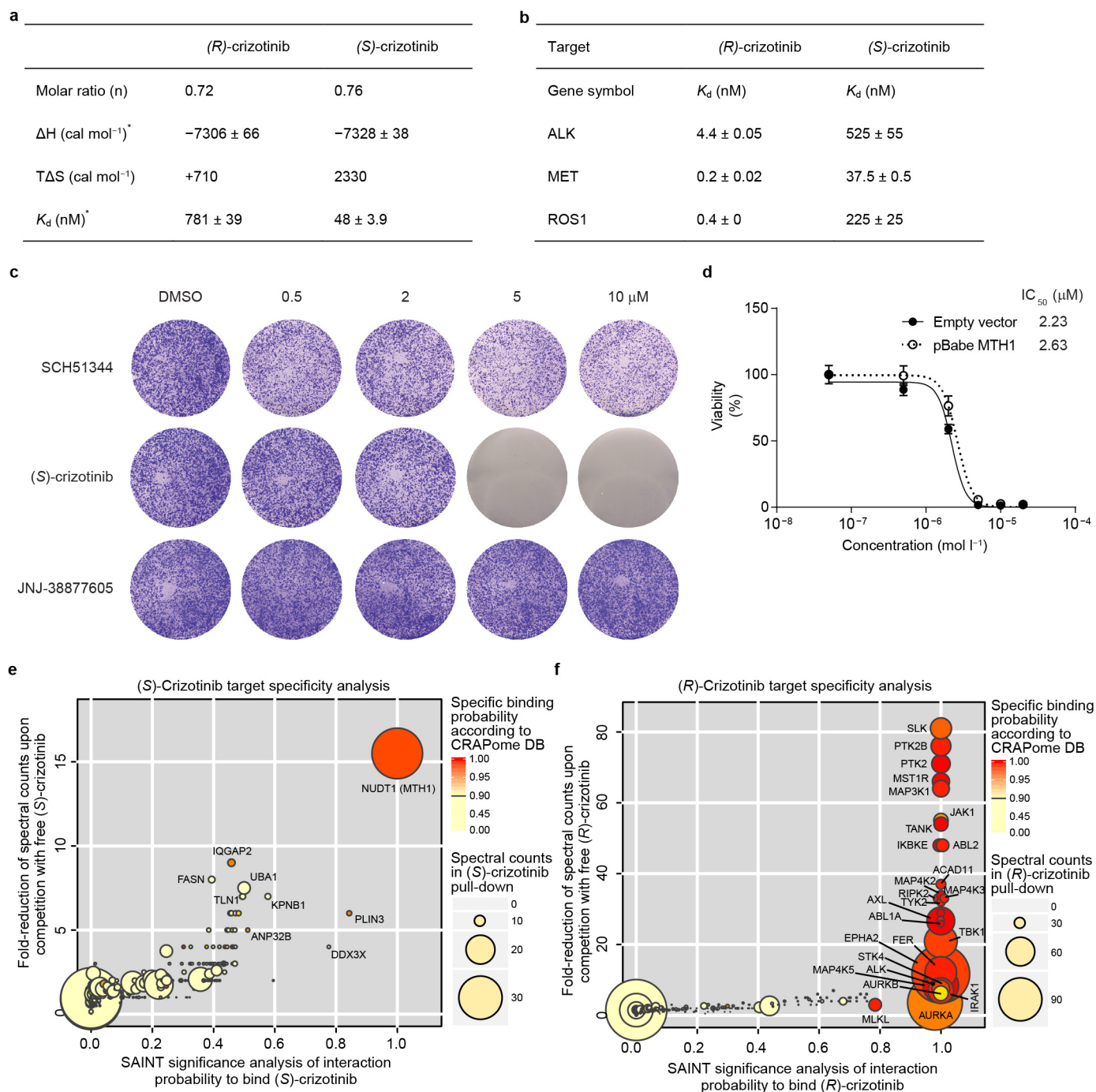
Extended Data Figure 2 | ( S )-Crizotinib target specificity. a , Isothermal titration calorimetry results for both crizotinib enantiomers. Data were measured at 15 °C in 50 mM Tris-HCl pH 7.8, 150 mM NaCl. *Error given in the table represent the error of the nonlinear least squares fit to the experimental data ( n = 1 ). b , K_d binding constants of both crizotinib enantiomers for the ( R )-crizotinib cognate targets ALK, MET and ROS1. Data are shown as mean ± s.e.m. ( n = 2 ). c , Pharmacologic c-MET kinase inhibition by a highly potent inhibitor (JNJ-38877605, c-MET IC_{50} = 4 nM) does not suppress growth of KRAS-mutated SW480 cells in contrast to the MTH1 inhibitors SCH51344 and ( S )-crizotinib. Images are representative of three independent experiments ( n = 3 ). d , MTH1 overexpression does not alter SW480 sensitivity towards ( S )-crizotinib. Data are shown as mean ± s.e.m. and
